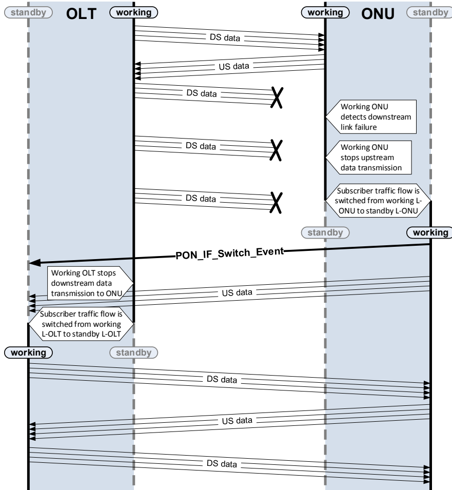
Figure 9-10—An example of tree protection switching: downstream link failure detected by working ONU
