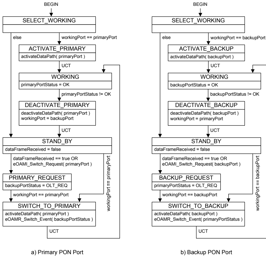
Figure 9-12—Tree protection process operating on the ONU
