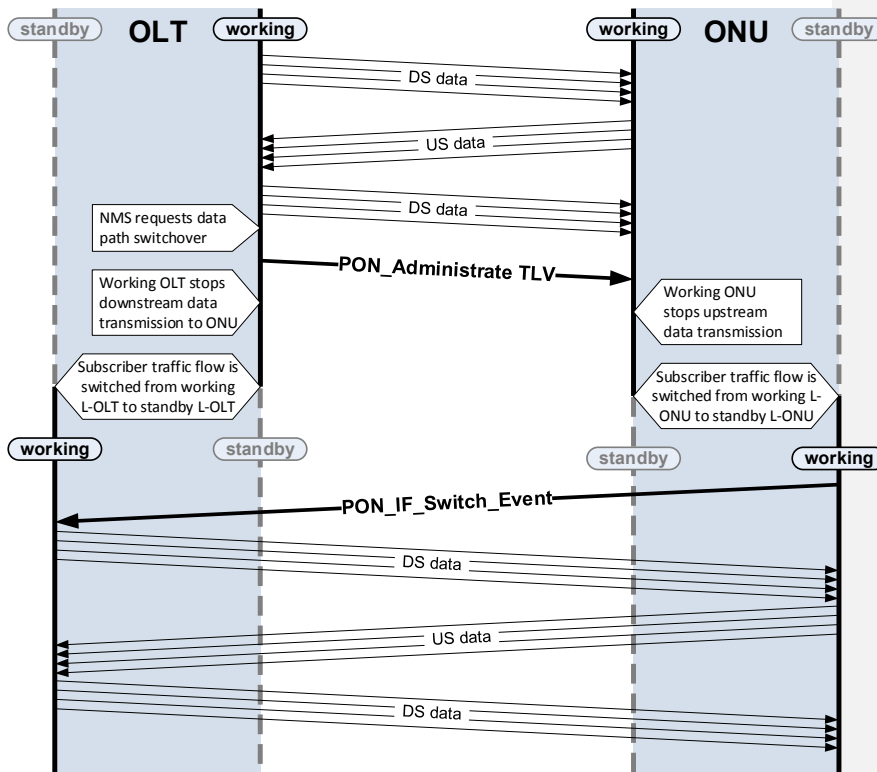
Figure 9-7—An example of tree protection switching: NMS driven request
