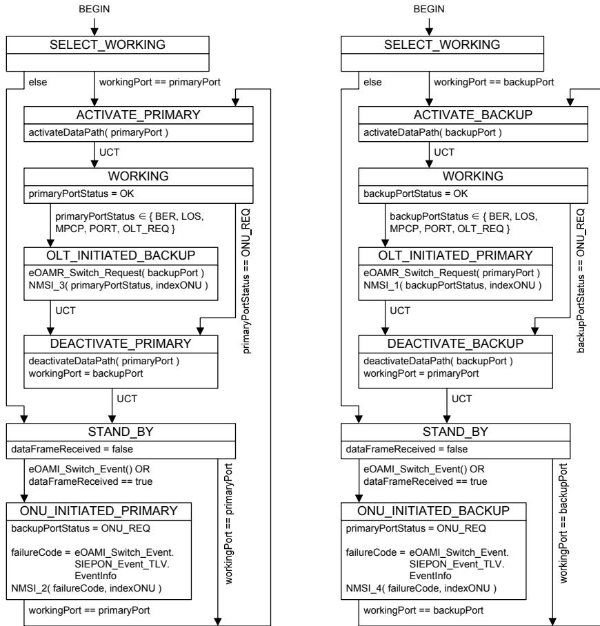
a) Primary PON Port
