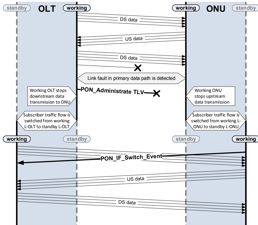
Figure 9-8—An example of tree protection switching: link failure detected by working OLT and working C-ONU
