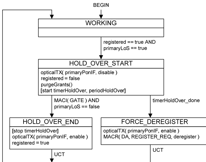
Figure 9-4—Trunk protection process operating on the ONU
