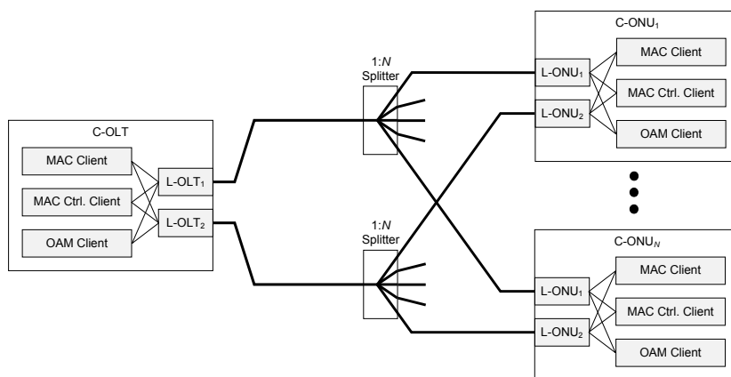
Figure 9-5—Tree protection with redundant L-OLT
