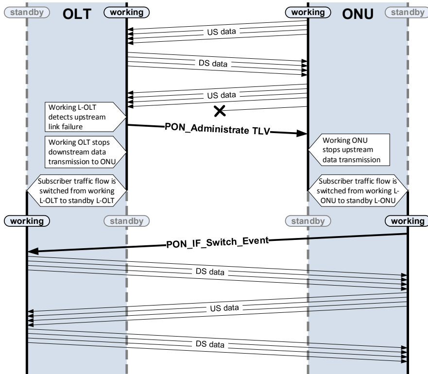
Figure 9-9—An example of tree protection switching: upstream link failure detected by working OLT
