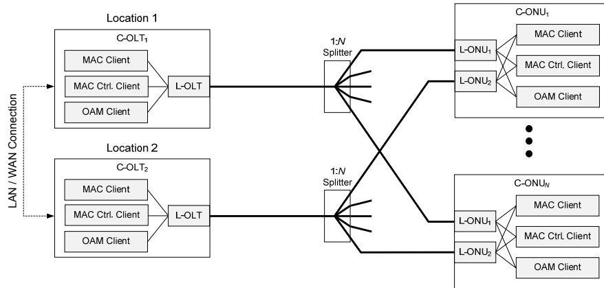
Figure 9-6—Tree protection with redundant C-OLT
