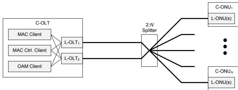
Figure 9-1—Trunk protection with redundant L-OLT
