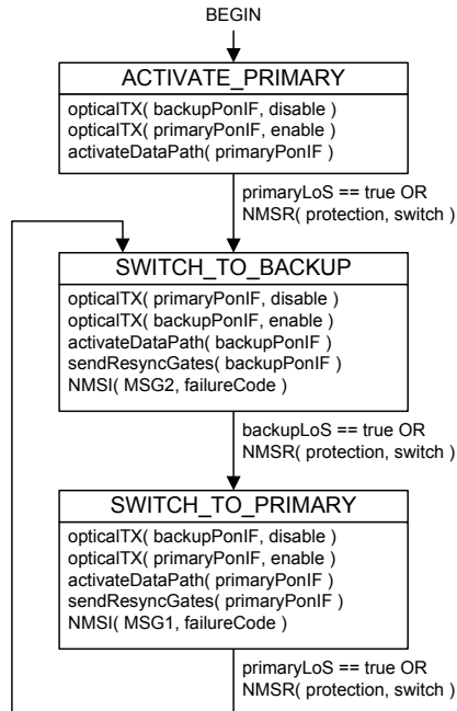
Figure 9-3—Trunk protection process operating on the OLT
