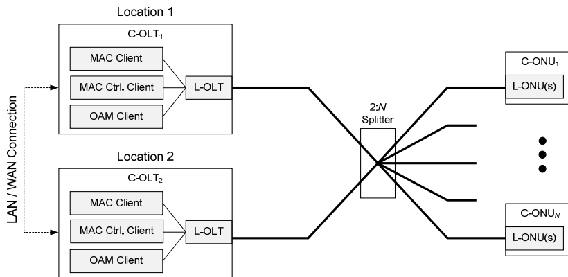
Figure 9-2—Trunk protection with redundant C-OLT
